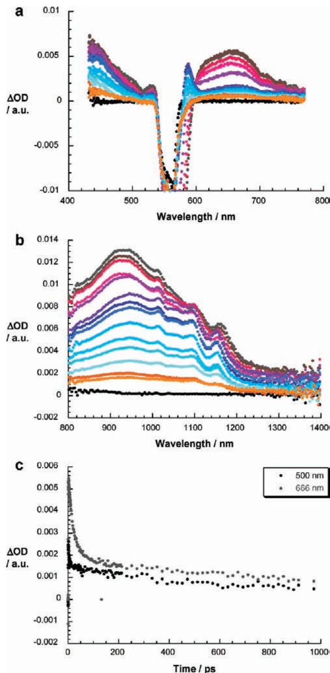
Figure 12. (a) Differential absorption spectra (visible) obtained upon femtosecond flash photolysis (550 nm, 150 nJ) of C_{60} -S-Fc-O in THF with several time delays between 0 and 1000 ps at room temperature; time evolution from black to red to blue and orange. (b) Differential absorption spectra (near-infrared) obtained upon femtosecond flash photolysis (550 nm, 150 nJ) of C_{60} -S-Fc-O in THF with several time delays between 0 and 1000 ps at room temperature; time evolution from black to red to blue and orange. (c) Time-absorption profiles of the spectra at 500 and 666 nm, monitoring the charge separation dynamics.
