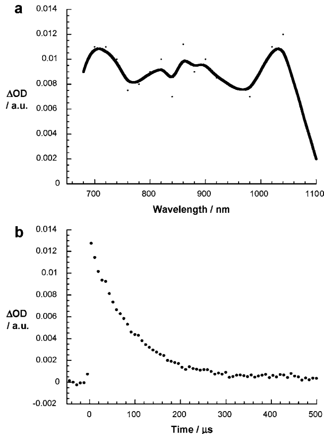
Figure 11. (a) Differential absorption spectrum (near-infrared) obtained upon nanosecond flash photolysis (535 nm, 150 nJ) of C 60 -S-Fc-Ca in THF with a time delay of 25 ns at room temperature. (b) Time-absorption profiles of the spectra at 1060 nm, monitoring the charge recombination dynamics.
