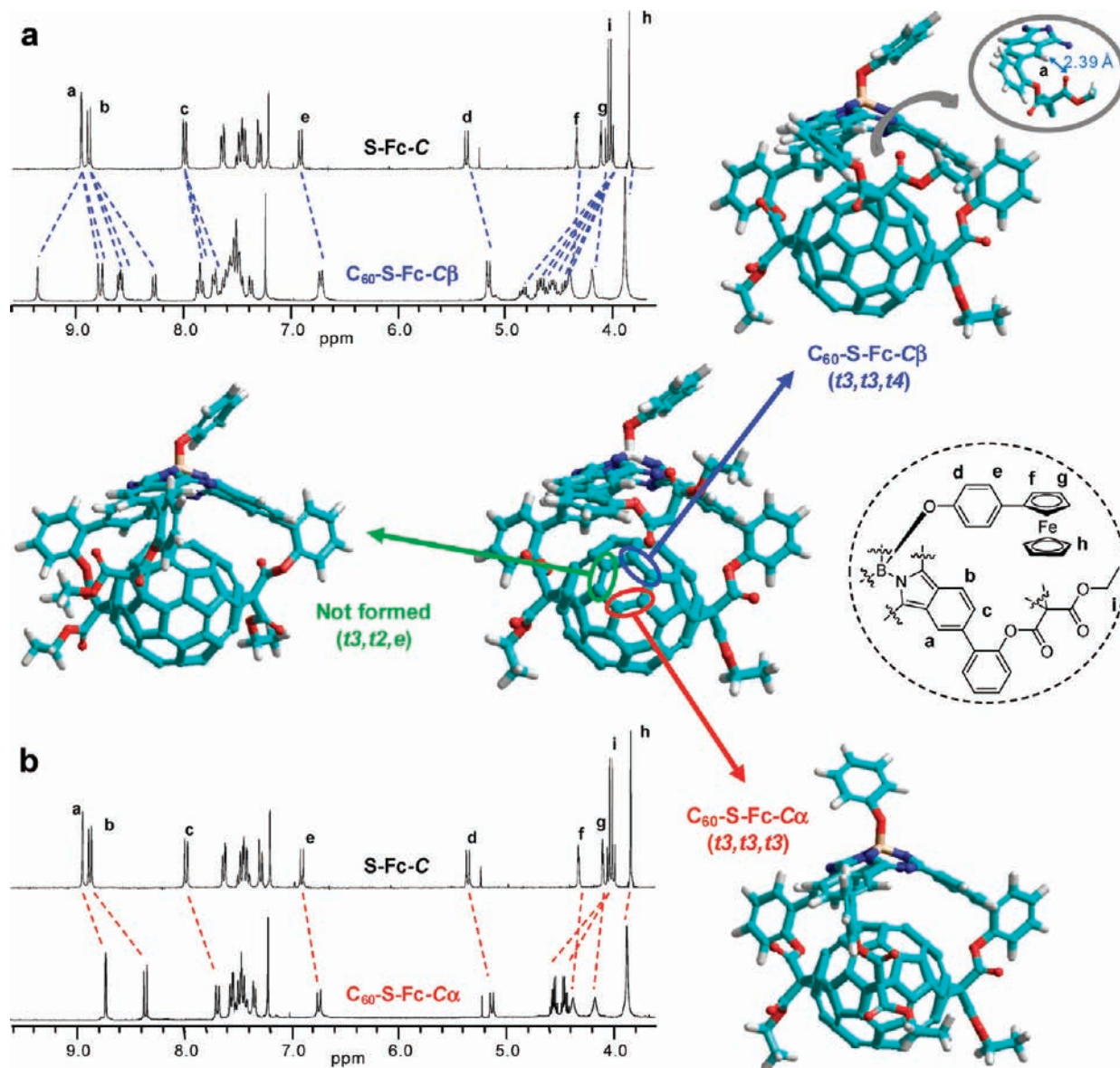
Figure 1. Scheme showing a model of a possible t_3 bisadduct intermediate formed during the triscyclopropanation reaction between S-Fc-C and C_{60} . The remaining third tether can then react with any of the circled double bonds, yielding the C_3 -symmetric t_3,t_3,t_3 trisadduct (in red; C_{60} - S-Fc-C \alpha ), or the C_1 -symmetric t_3,t_3,t_4 (in blue; C_{60} - S-Fc-C \beta ) or t_3,t_2,e (in green; not formed) trisadducts, whose models are also displayed (the ferrocene unit has been omitted). (a) ^1\text{H} NMR spectra ( \text{CDCl}_3 , 298 K, 500 MHz) of compound C_{60} - S-Fc-C \beta compared to the S-Fc-C precursor. The unusual downfield shift of one of the proton “a” signals may be explained by a spacer conformation in which a carbonyl group is close to this isoindole proton, as shown in the magnification of the C_{60} - S-Fc-C \beta model, which supports our assignment. (b) ^1\text{H} NMR spectra ( \text{CDCl}_3 , 298 K, 500 MHz) of compound C_{60} - S-Fc-C \alpha compared to the S-Fc-C precursor.
