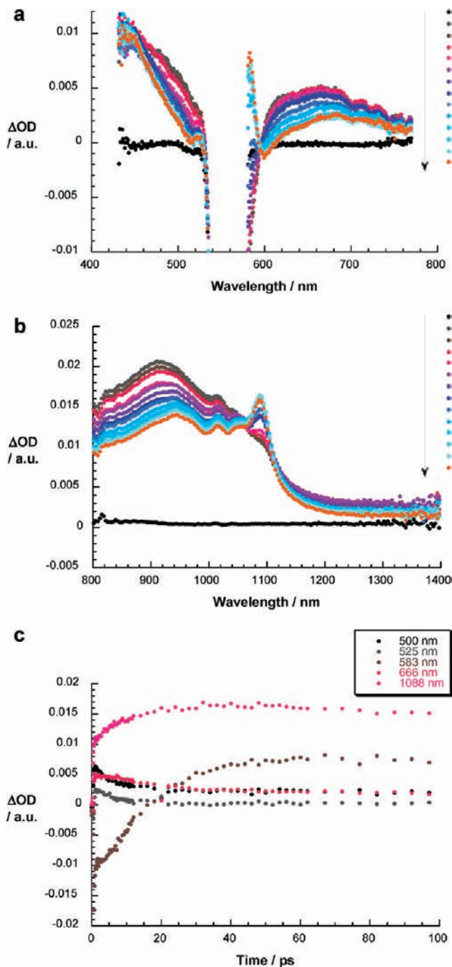
Figure 10. (a) Differential absorption spectra (visible) obtained upon femtosecond flash photolysis (550 nm, 150 nJ) of C 60 -S-Fc-Ca in THF with several time delays between 0 and 100 ps at room temperature; see figure legend for time evolution. (b) Differential absorption spectra (near-infrared) obtained upon femtosecond flash photolysis (550 nm, 150 nJ) of C 60 -S-Fc-Ca in THF with several time delays between 0 and 100 ps at room temperature; see figure legend for time evolution. (c) Time-absorption profiles of the spectra at 500, 525, 583, 666, and 1088 nm, monitoring the charge separation dynamics.
