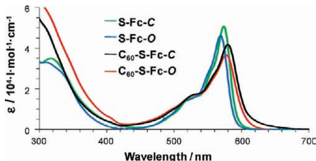
Figure 3. Electronic absorption spectra ( \text{CHCl}_3 , c = 10^{-5} M) of \text{C}_{60}\text{-S-Fc-C}\alpha and \text{C}_{60}\text{-S-Fc-O} compared to SubPc–Fc \text{S-Fc-C} and \text{S-Fc-O} .
