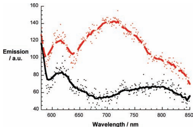
Figure 6. Room temperature steady-state fluorescence spectra of \text{C}_{60}-\text{S}-\text{C}\alpha (black spectrum) and \text{C}_{60}-\text{S}-\text{O} (red spectrum) in THF upon 560 nm excitation.
